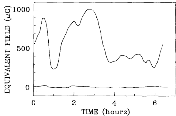
Figure 3. Evolution of trapped magnetic dipole moment before (upper trace) and after flux flushing (lower trace). Dipole magnitude expressed in units of equivalent uniform field in the sphere.
