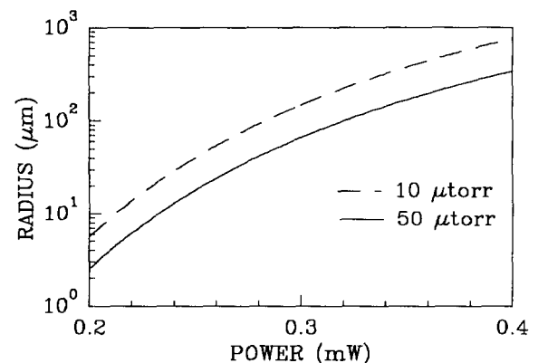
Figure 1. Hot spot radius versus power into film.
